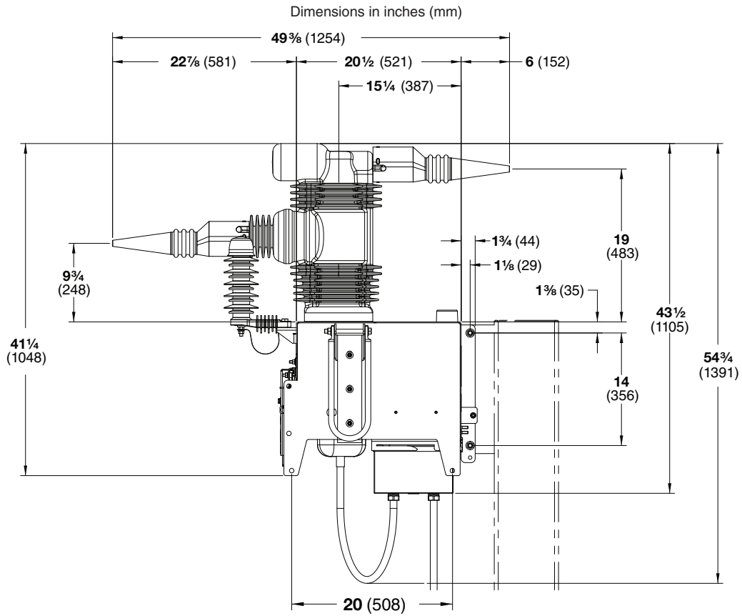
SIDE VIEW
