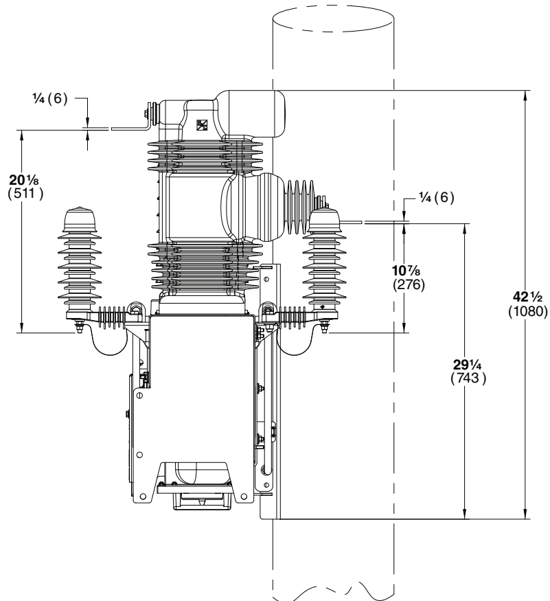
SIDE VIEW
