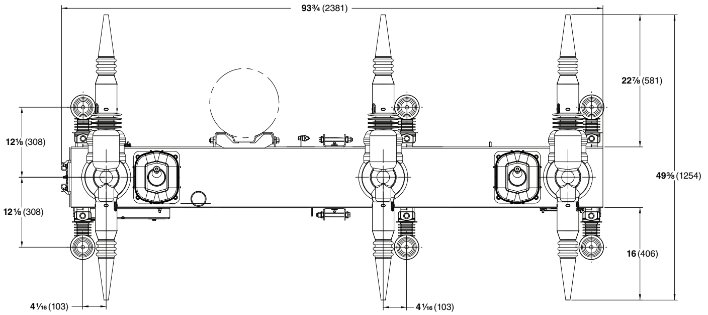
TOP VIEW
