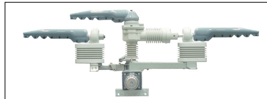
Figure 3. The wildlife protection helps reduce wildlife-related nuisance outages.
