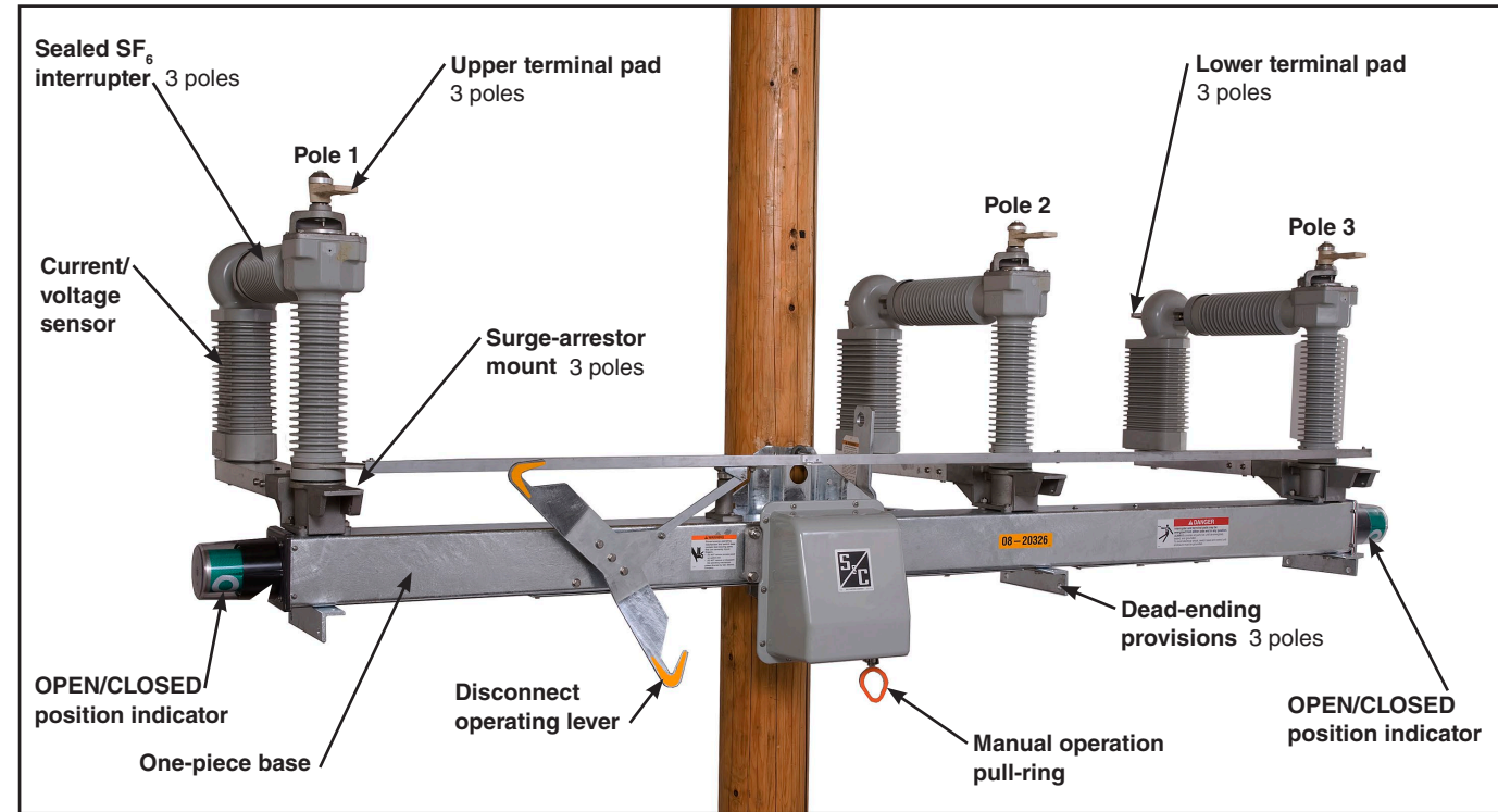
Figure 1. The Scada-Mate Switching System Upright Mounting Configuration.
