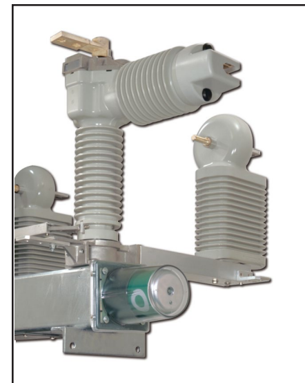
Figure 2. The visible disconnect in the Open position.
