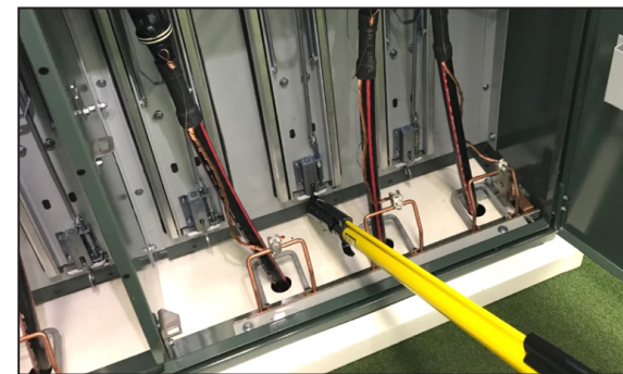
Figure 5. Unlatching (or latching) a TransFuser Mounting in the Closed position.
