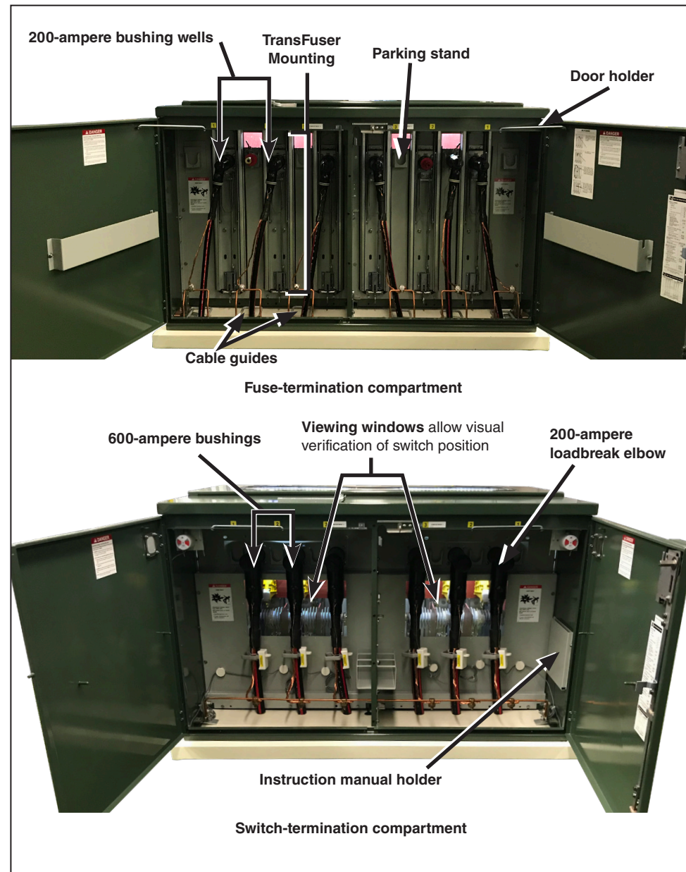
Figure 1. The manual Model PME-9 showing open-door views of fuse-termination compartments and switch-termination compartments.
