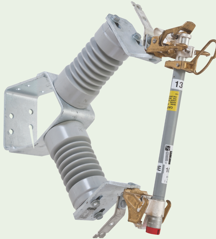
FIGURE 24. 14.4-kV Station—Right-Angle Style
