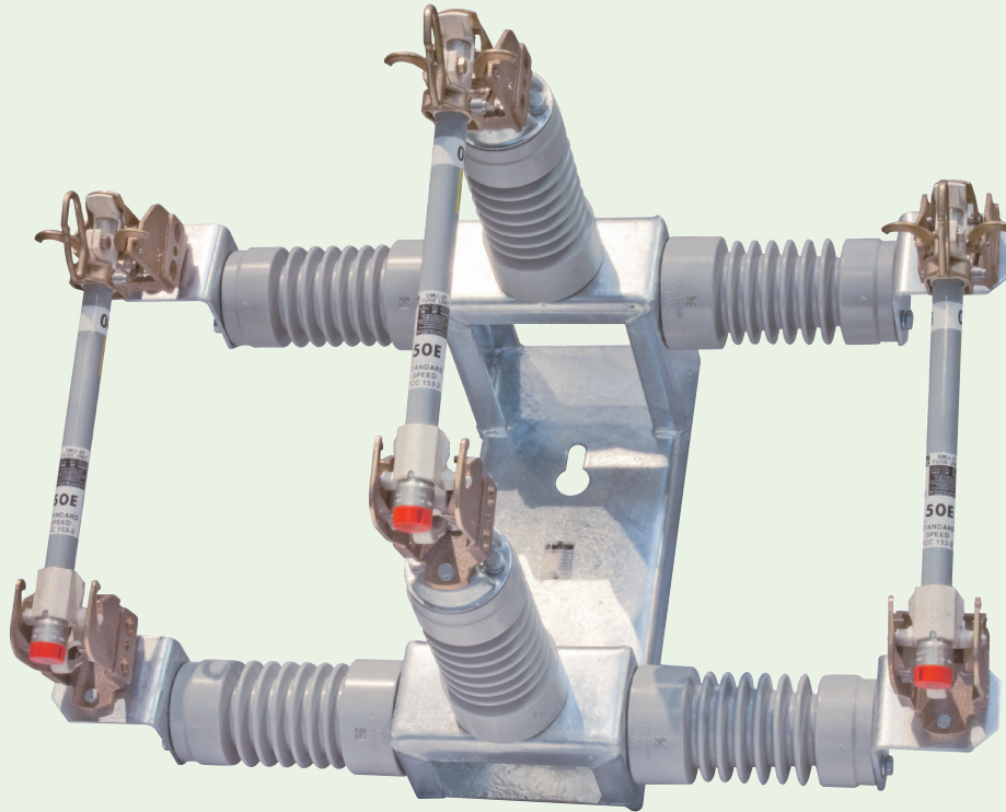
FIGURE 25. 14.4-kV Station—Cluster-Offset Style
