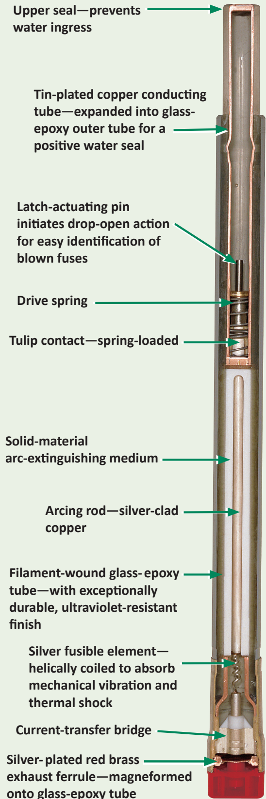
FIGURE 8. An inside view of the SMU-20 Fuse Unit.
