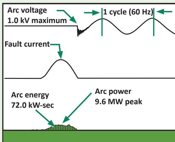
FIGURE 2. The arc energy of an SMD-20 Power Fuse.
