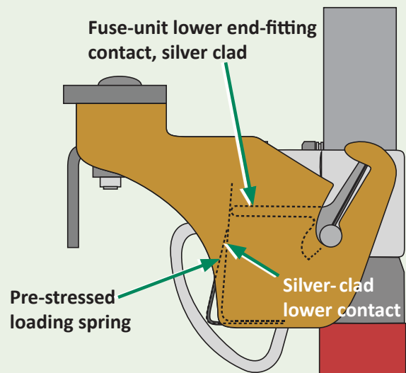
FIGURE 7. Lower contacts—silver-to-silver—provide a dual current path independent of the hinge pivot.
