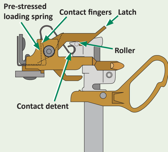
FIGURE 6. The latch-and-upper-contact assembly (fully closed).
