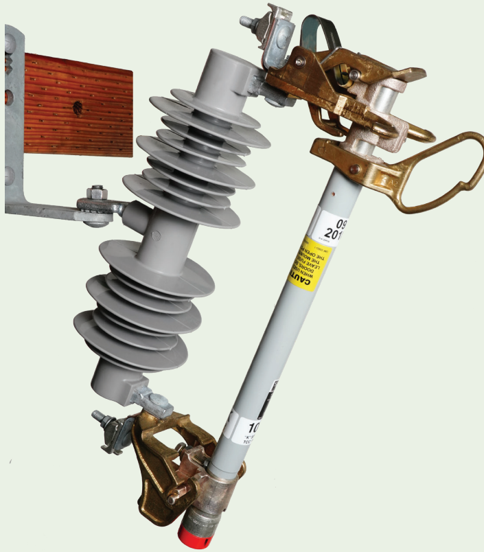
FIGURE 20. 14.4-kV Overhead—Pole-Top Style
