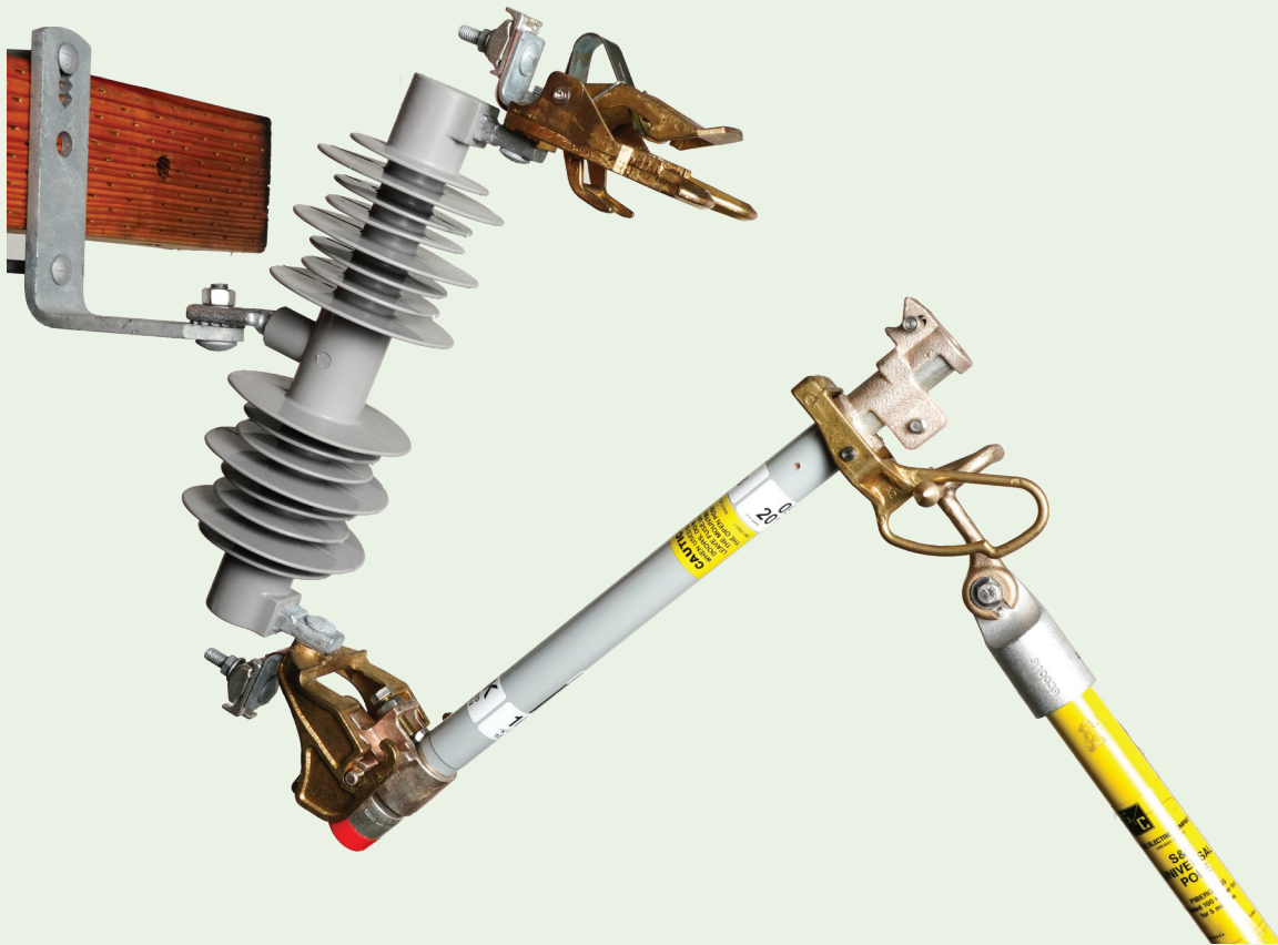
FIGURE 16. Closing the fuse unit.
